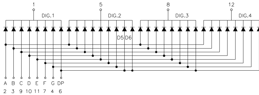
Common Cathode
